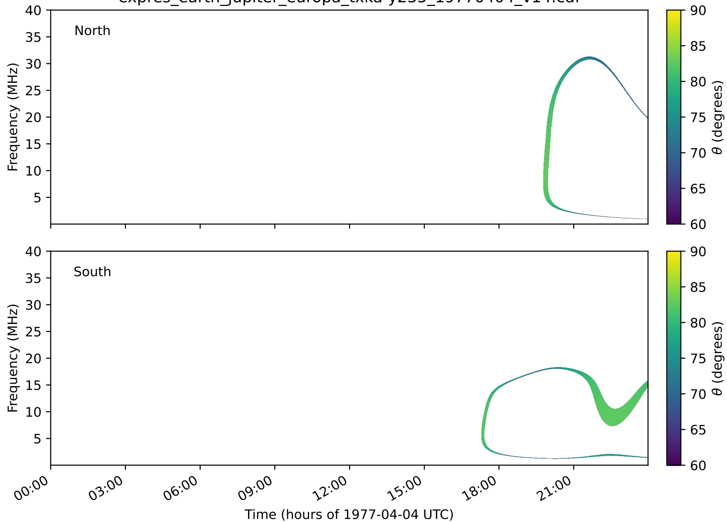
expres_earth_jupiter_europa_txka-y235_19770404_v14.cdf
