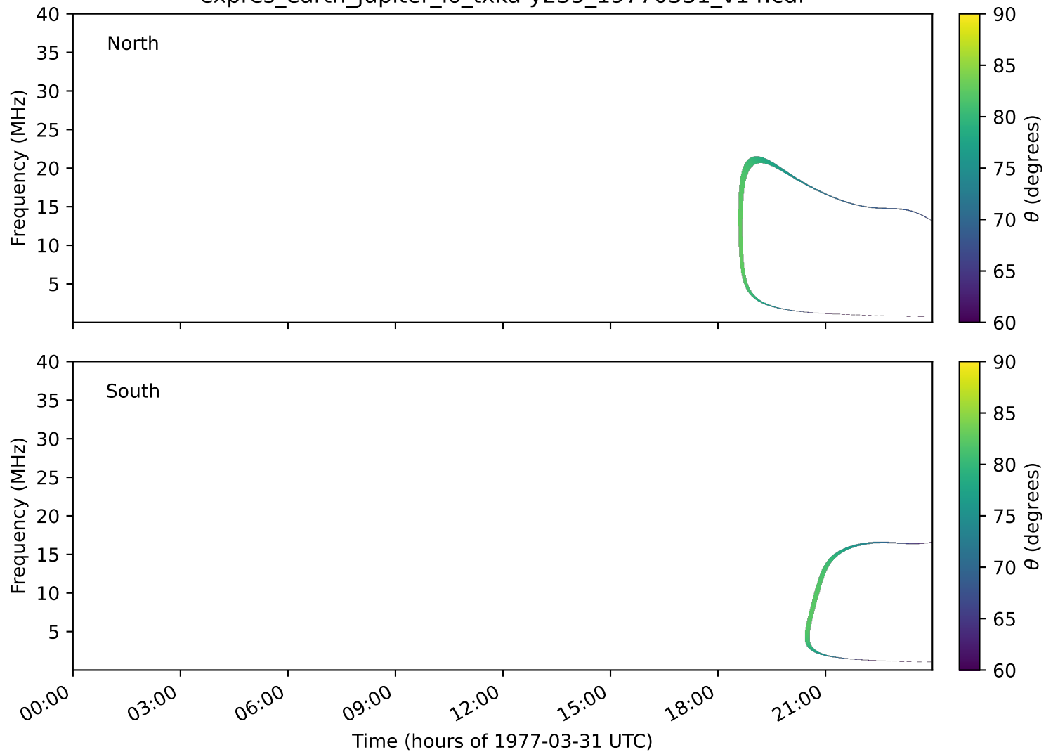
expres_earth_jupiter_io_txka-y235_19770331_v14.cdf
