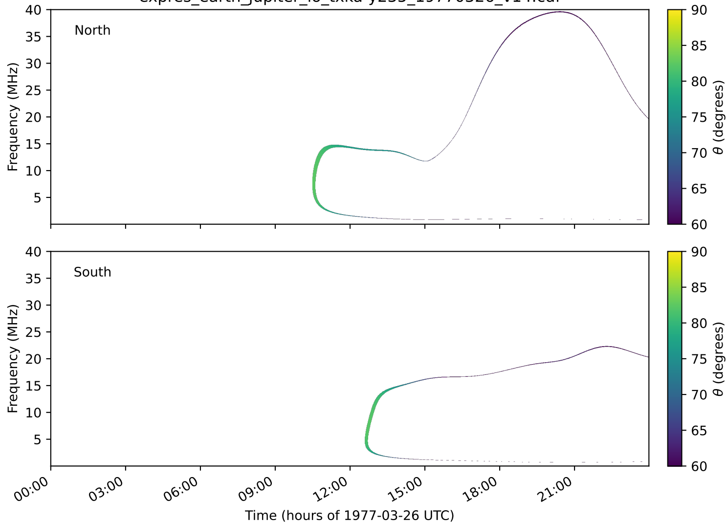
expres_earth_jupiter_io_txka-y235_19770326_v14.cdf
