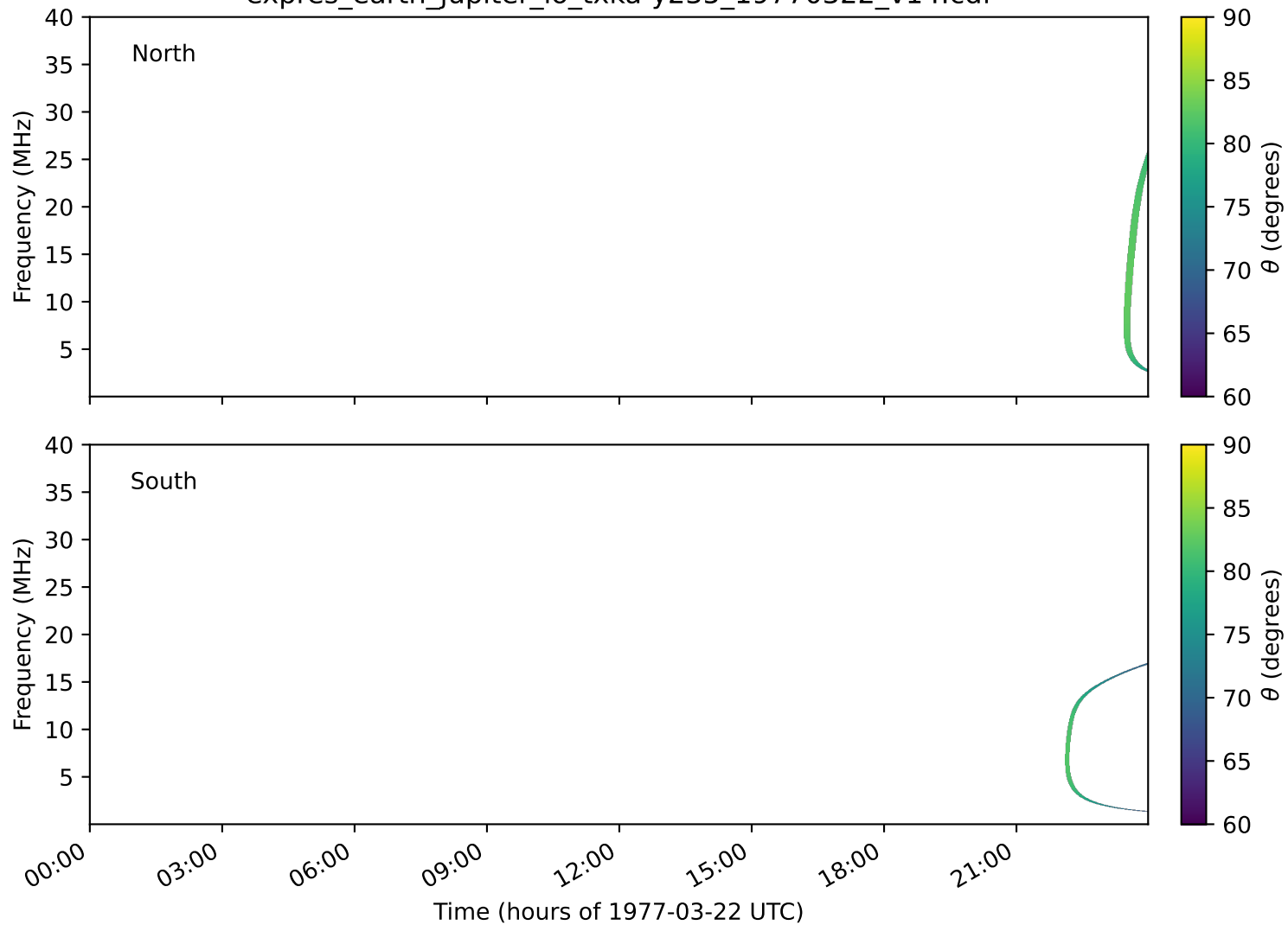
expres_earth_jupiter_io_txka-y235_19770322_v14.cdf
