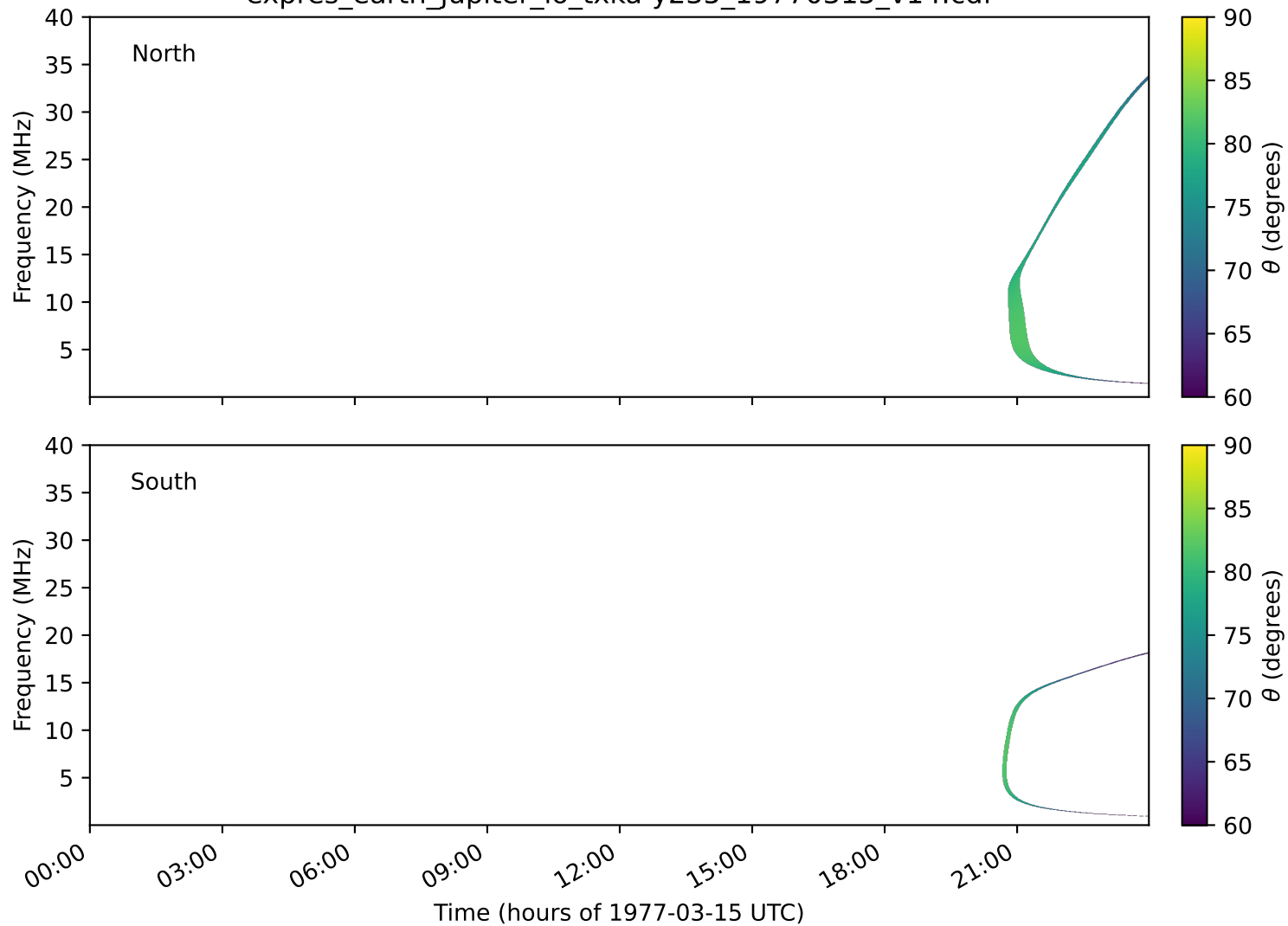
expres_earth_jupiter_io_txka-y235_19770315_v14.cdf
