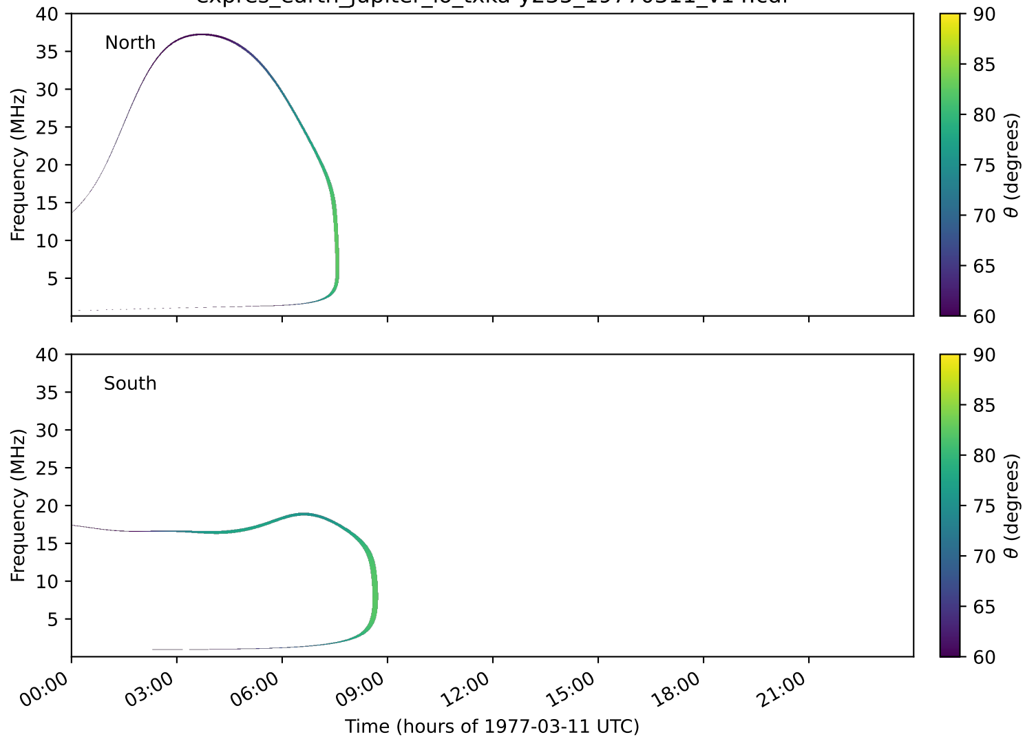
expres_earth_jupiter_io_txka-y235_19770311_v14.cdf
