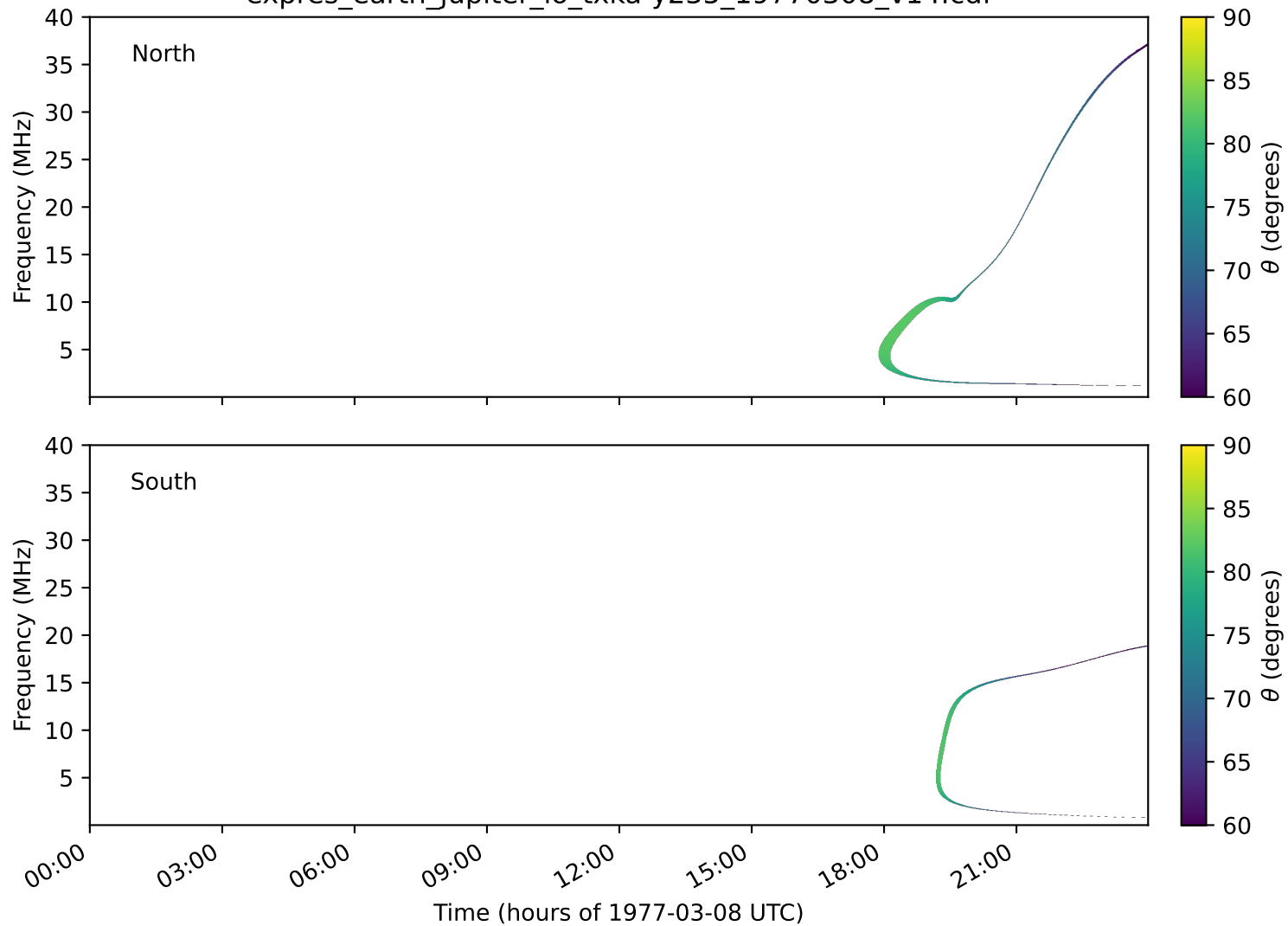
expres_earth_jupiter_io_txka-y235_19770308_v14.cdf
