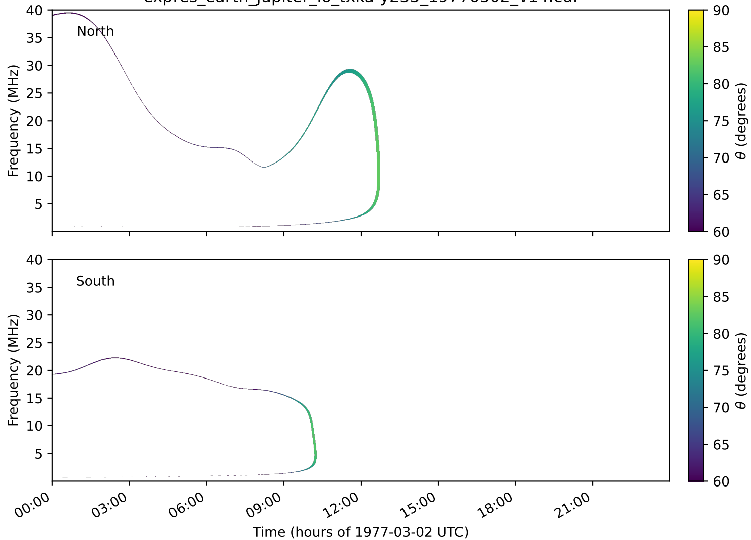
expres_earth_jupiter_io_txka-y235_19770302_v14.cdf
