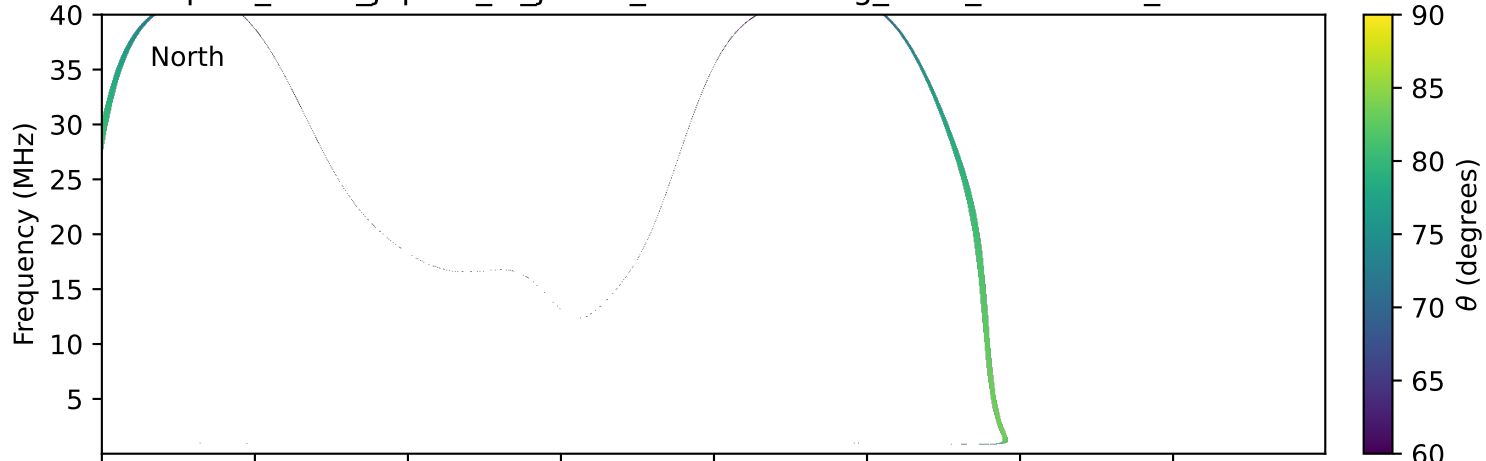
expres_earth_jupiter_io_jrm33_lossc-wid1deg_3kev_19770323_v11.cdf
