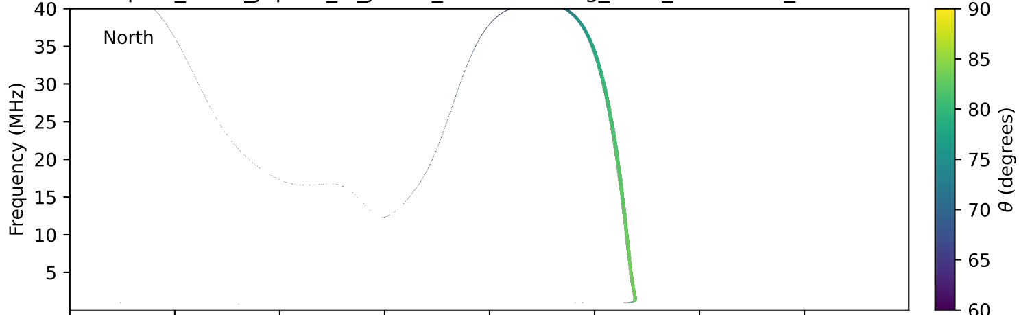
expres_earth_jupiter_io_jrm33_lossc-wid1deg_3kev_19770316_v11.cdf
