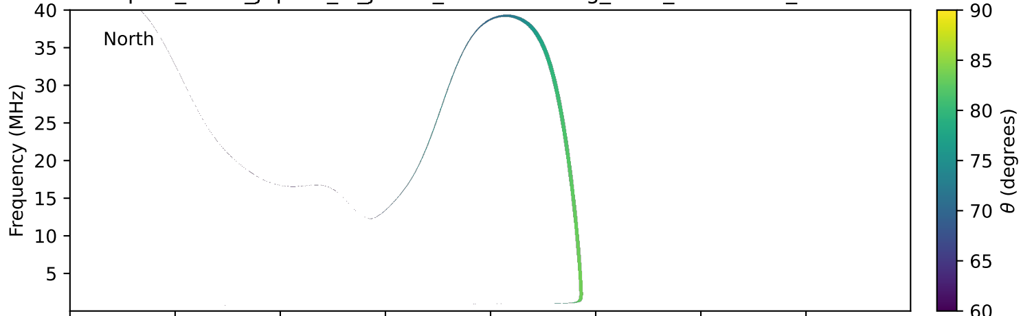
expres_earth_jupiter_io_jrm33_lossc-wid1deg_3kev_19770309_v11.cdf
