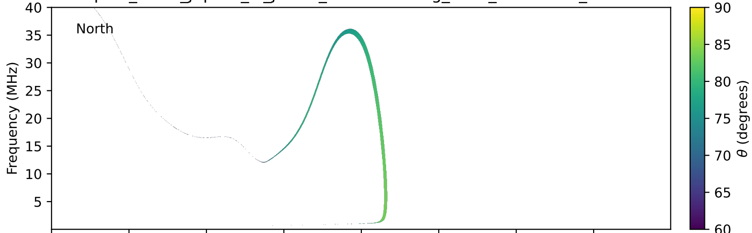
expres_earth_jupiter_io_jrm33_lossc-wid1deg_3kev_19770302_v11.cdf
