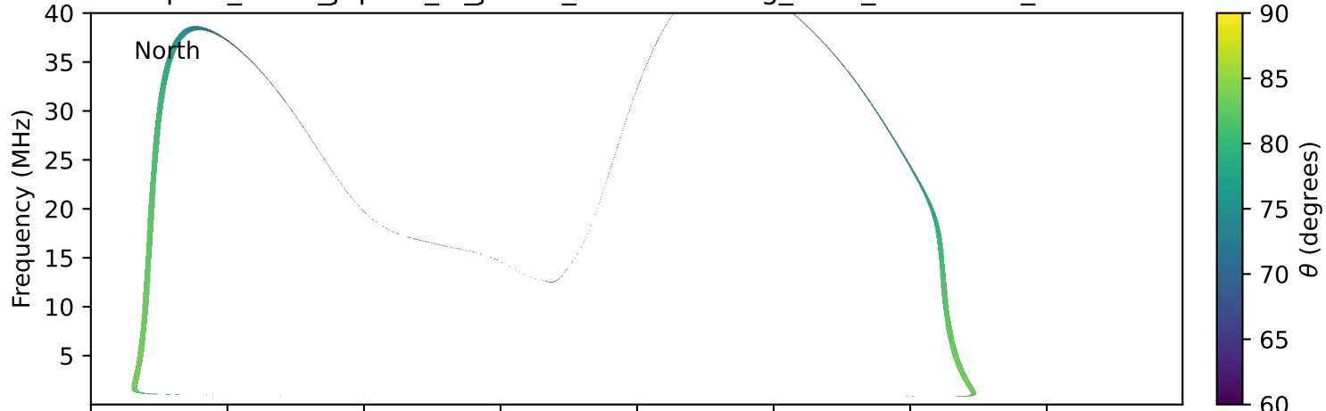
expres_earth_jupiter_io_jrm09_lossc-wid1deg_3kev_19770330_v11.cdf
