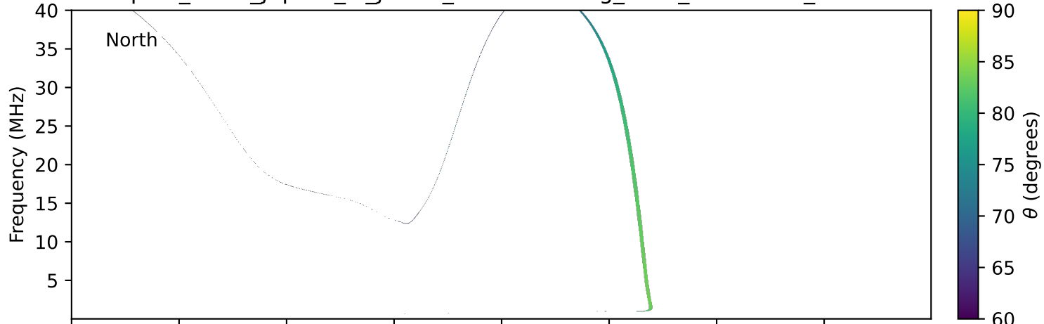
expres_earth_jupiter_io_jrm09_lossc-wid1deg_3kev_19770316_v11.cdf
