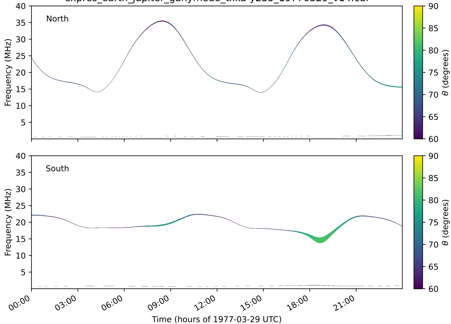
expres_earth_jupiter_ganymede_txka-y235_19770329_v14.cdf
