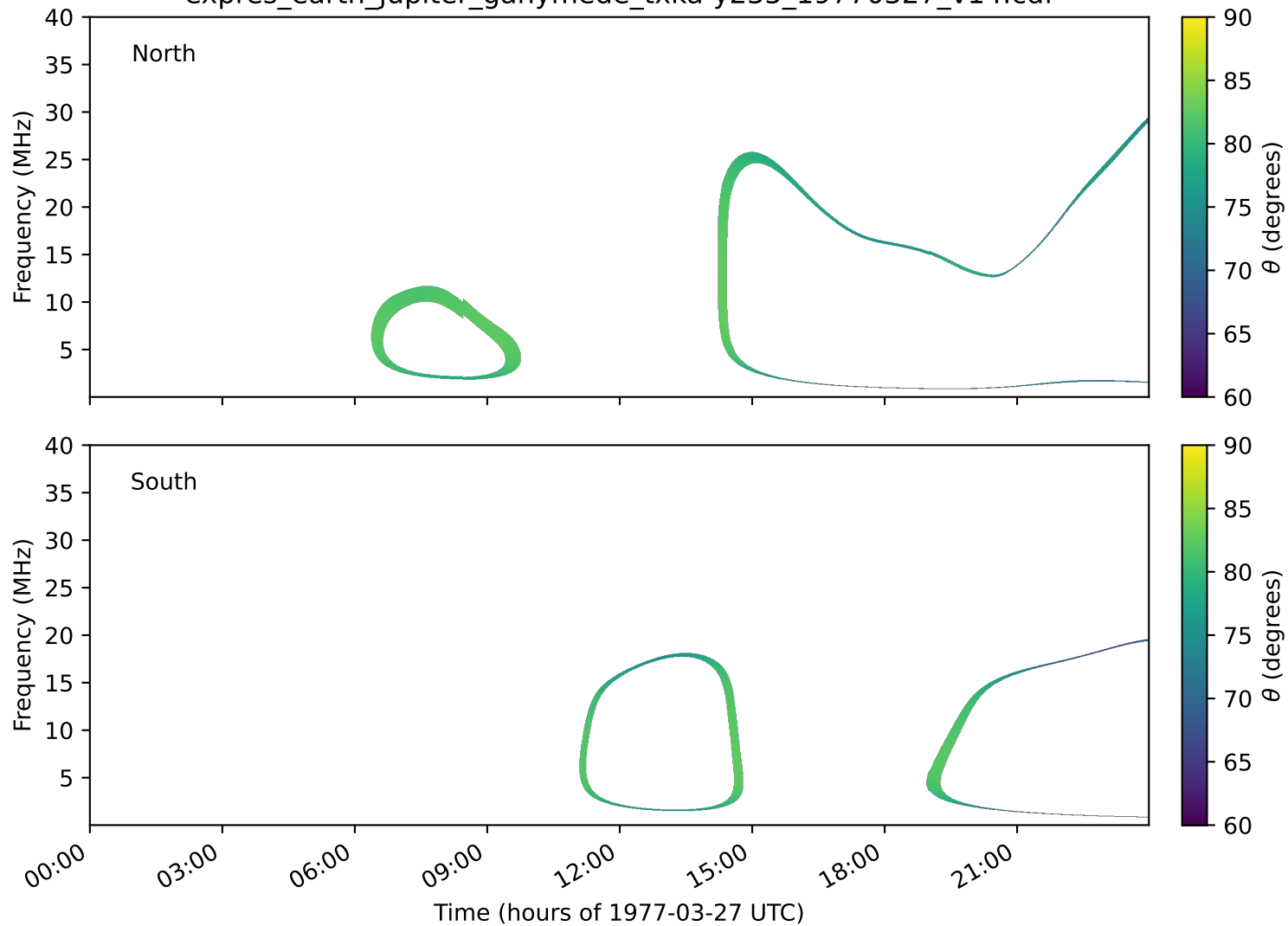
expres_earth_jupiter_ganymede_txka-y235_19770327_v14.cdf
