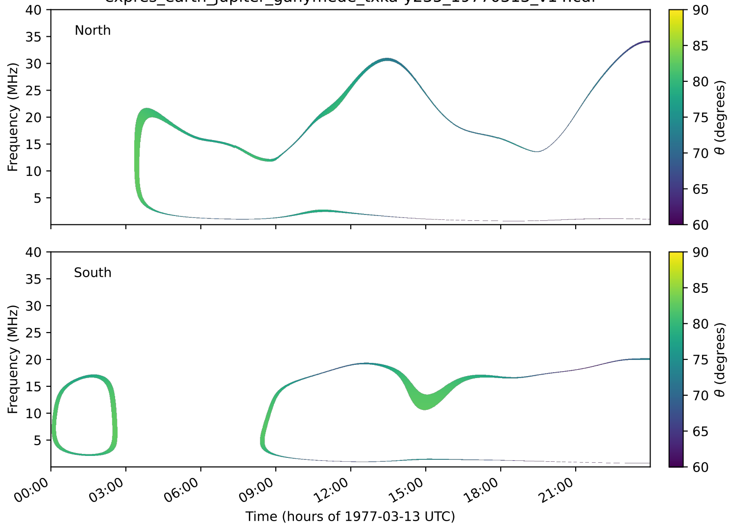
expres_earth_jupiter_ganymede_txka-y235_19770313_v14.cdf
