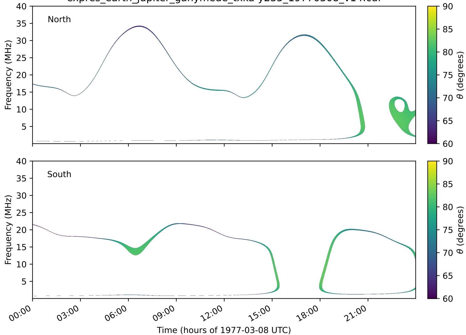
expres_earth_jupiter_ganymede_txka-y235_19770308_v14.cdf
