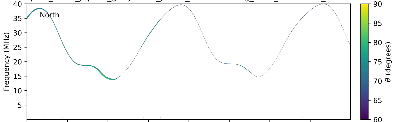
expres_earth_jupiter_ganymede_jrm33_lossc-wid1deg_3kev_19770328_v11.cdf
