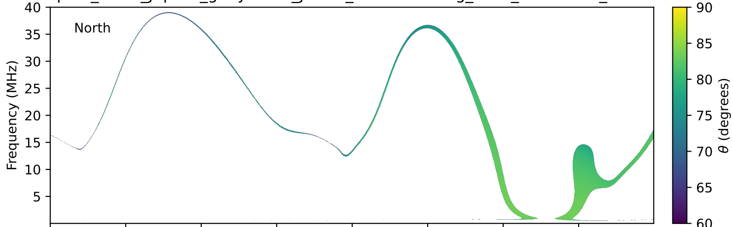
expres_earth_jupiter_ganymede_jrm09_lossc-wid1deg_3kev_19770330_v11.cdf
