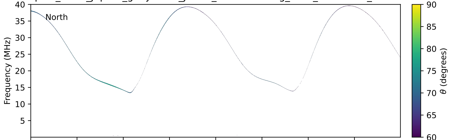
expres_earth_jupiter_ganymede_jrm09_lossc-wid1deg_3kev_19770321_v11.cdf
