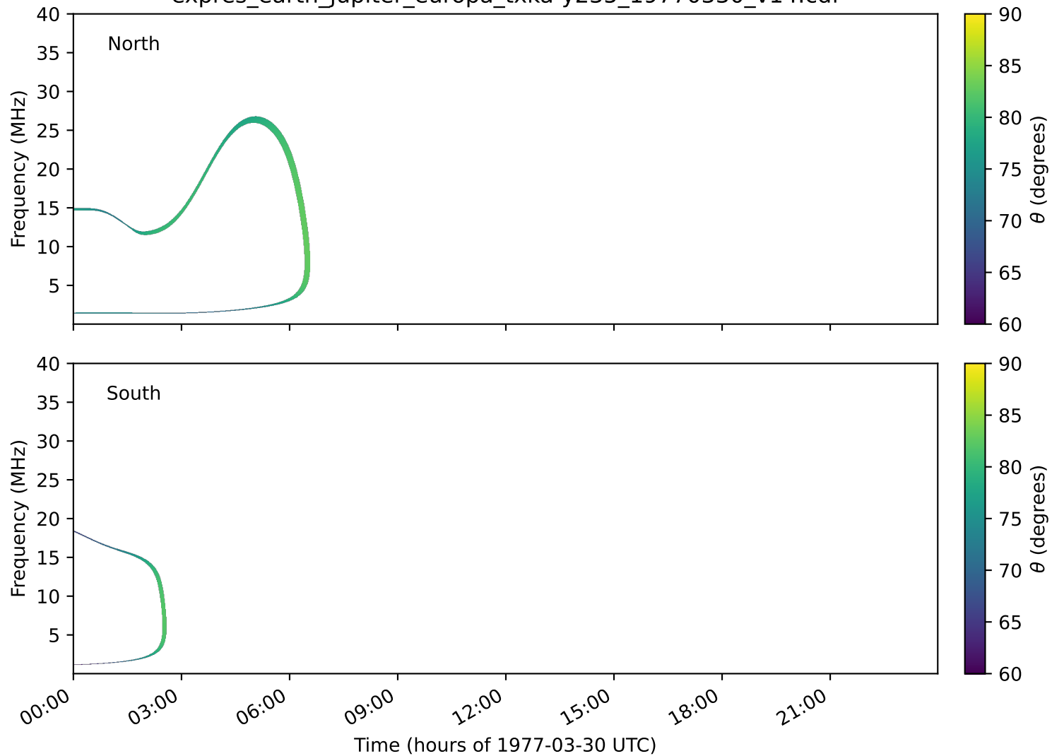
expres_earth_jupiter_europa_txka-y235_19770330_v14.cdf
