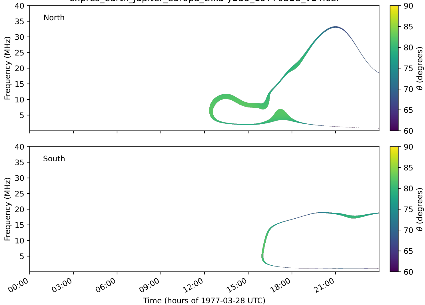
expres_earth_jupiter_europa_txka-y235_19770328_v14.cdf
