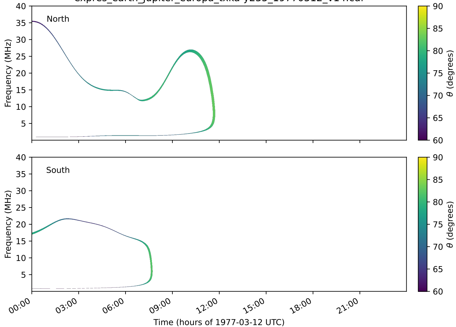
expres_earth_jupiter_europa_txka-y235_19770312_v14.cdf
