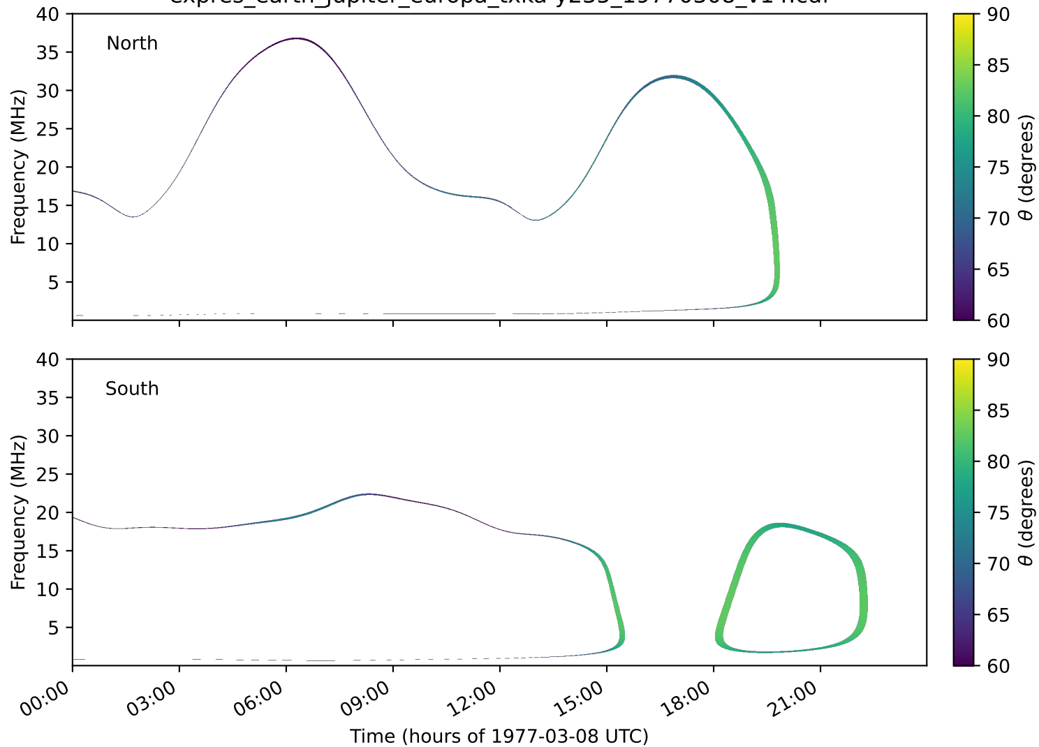
expres_earth_jupiter_europa_txka-y235_19770308_v14.cdf
