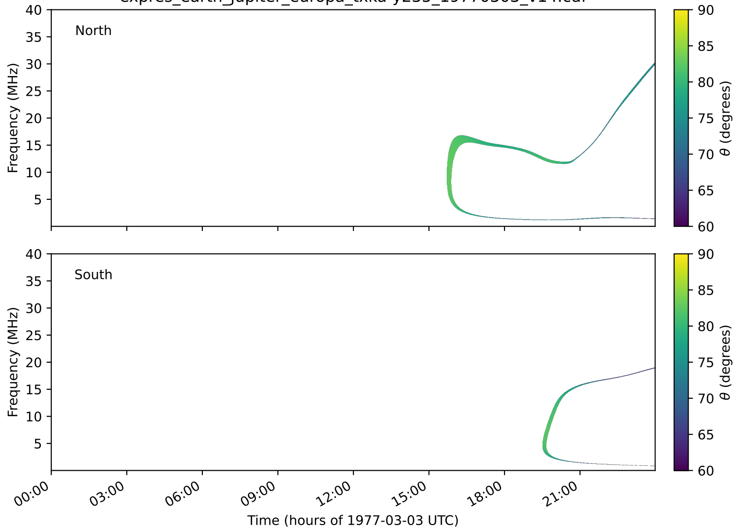
expres_earth_jupiter_europa_txka-y235_19770303_v14.cdf
