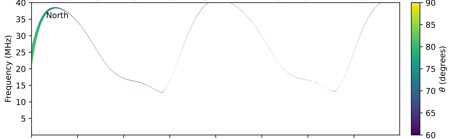
expres_earth_jupiter_europa_jrm09_lossc-wid1deg_3kev_19770311_v11.cdf
