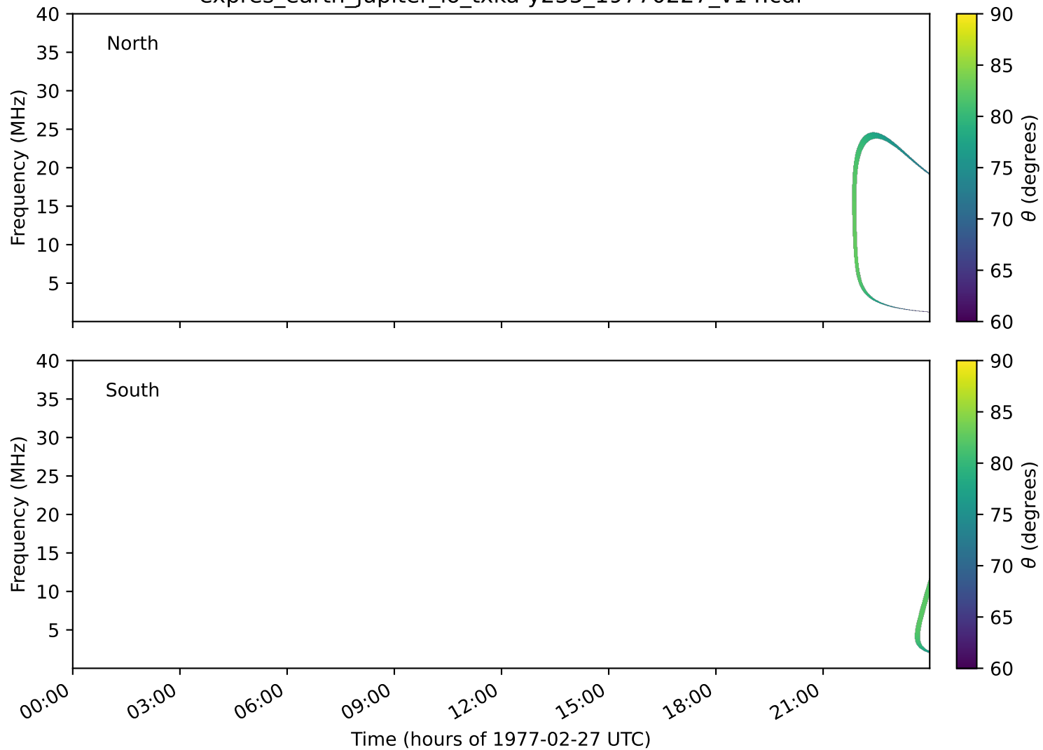
expres_earth_jupiter_io_txka-y235_19770227_v14.cdf
