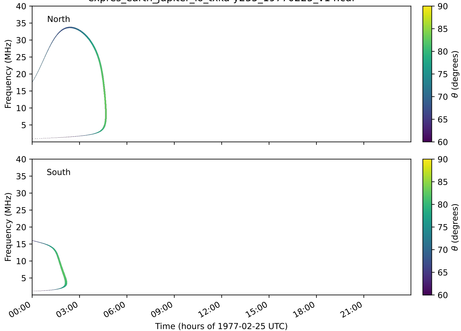
expres_earth_jupiter_io_txka-y235_19770225_v14.cdf
