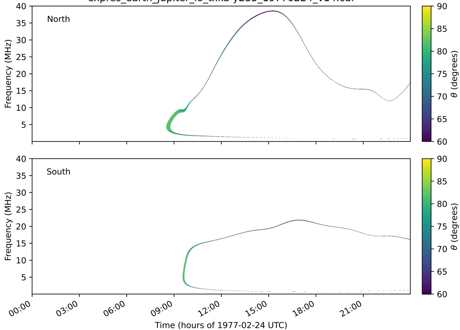
expres_earth_jupiter_io_txka-y235_19770224_v14.cdf
