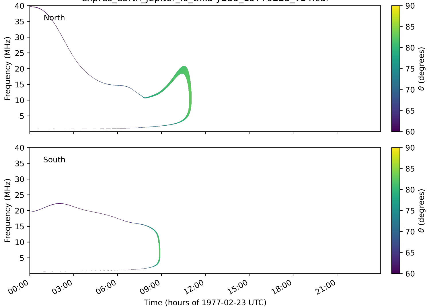
expres_earth_jupiter_io_txka-y235_19770223_v14.cdf
