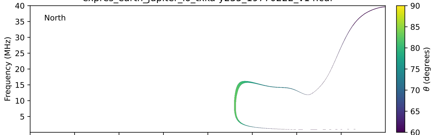
expres_earth_jupiter_io_txka-y235_19770222_v14.cdf
