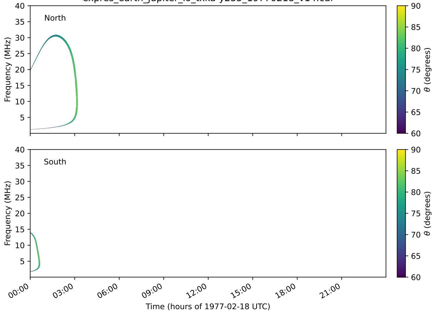
expres_earth_jupiter_io_txka-y235_19770218_v14.cdf
