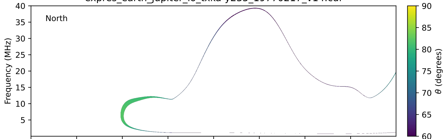
expres_earth_jupiter_io_txka-y235_19770217_v14.cdf
