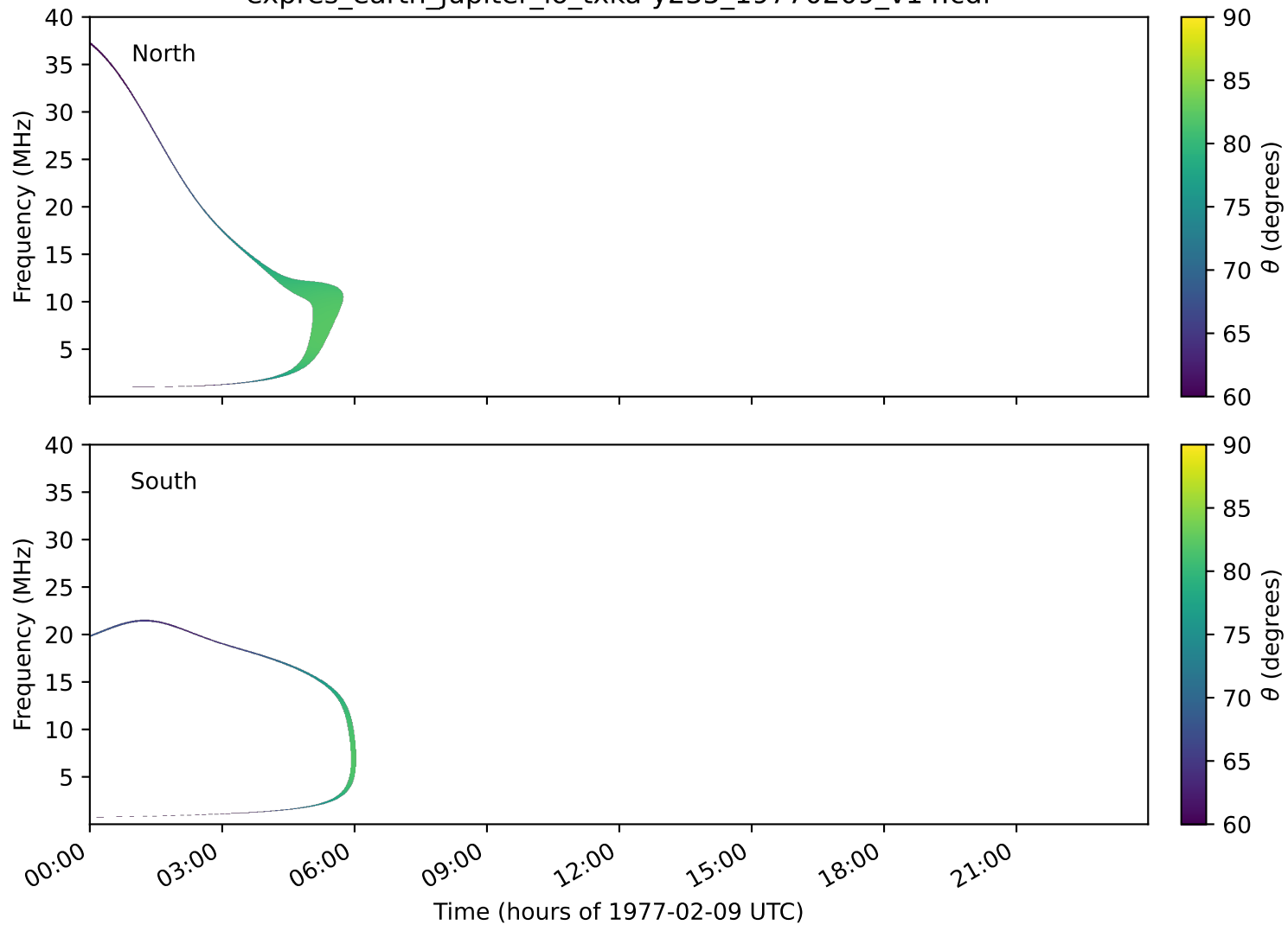
expres_earth_jupiter_io_txka-y235_19770209_v14.cdf
