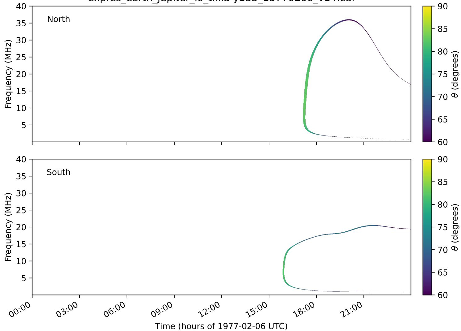
expres_earth_jupiter_io_txka-y235_19770206_v14.cdf
