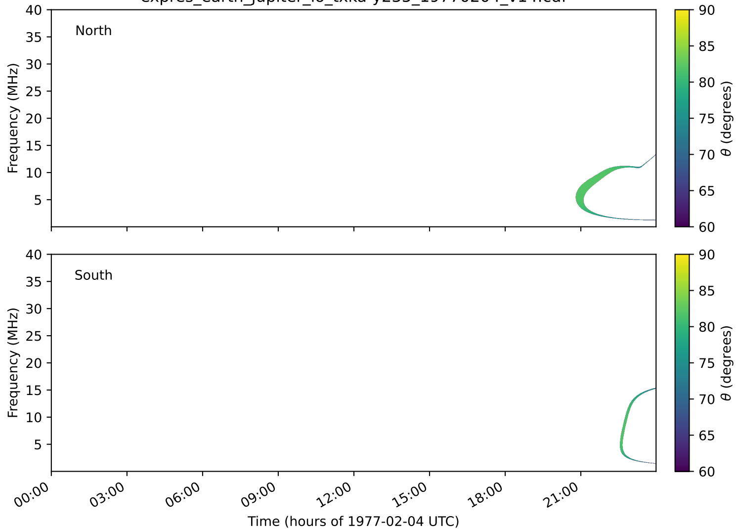
expres_earth_jupiter_io_txka-y235_19770204_v14.cdf
