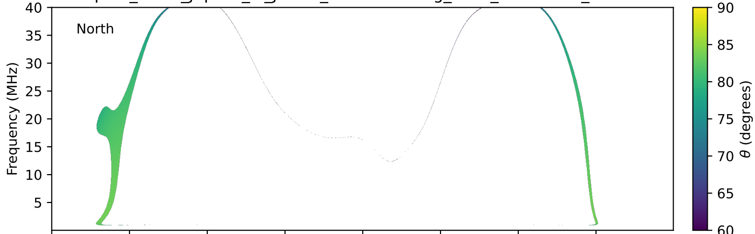
expres_earth_jupiter_io_jrm33_lossc-wid1deg_3kev_19770219_v11.cdf
