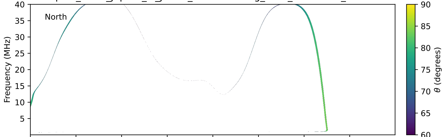
expres_earth_jupiter_io_jrm33_lossc-wid1deg_3kev_19770212_v11.cdf
