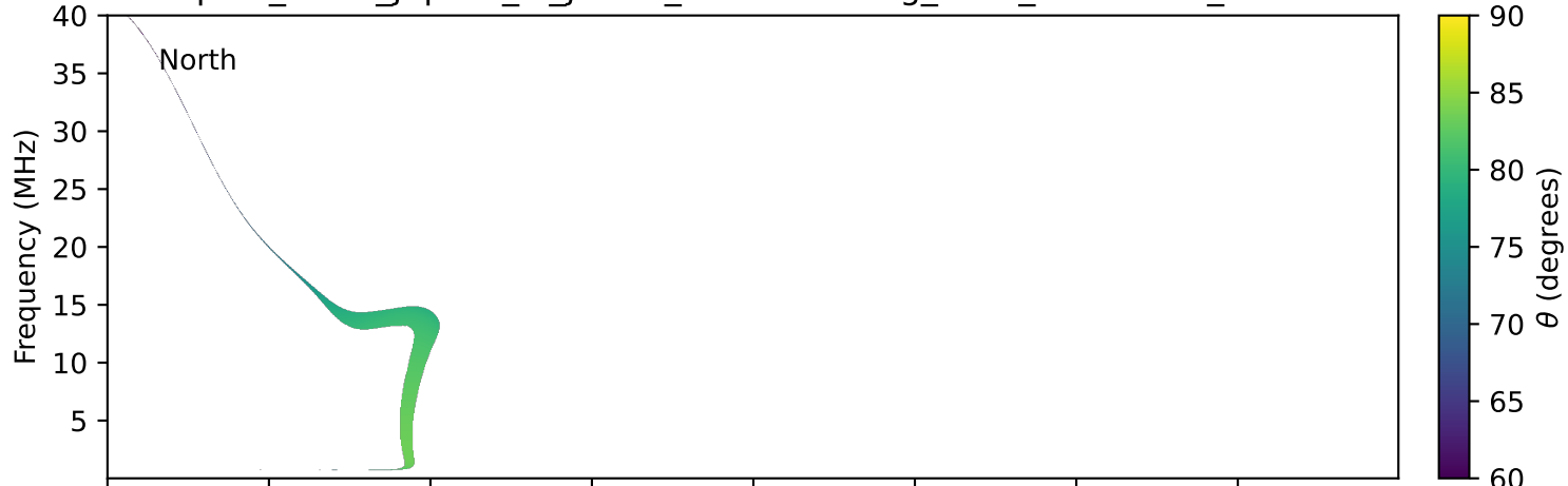
expres_earth_jupiter_io_jrm33_lossc-wid1deg_3kev_19770209_v11.cdf
