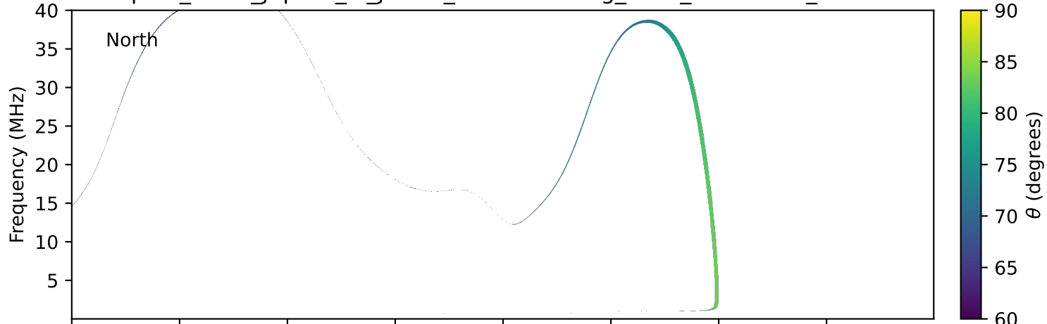
expres_earth_jupiter_io_jrm33_lossc-wid1deg_3kev_19770205_v11.cdf
