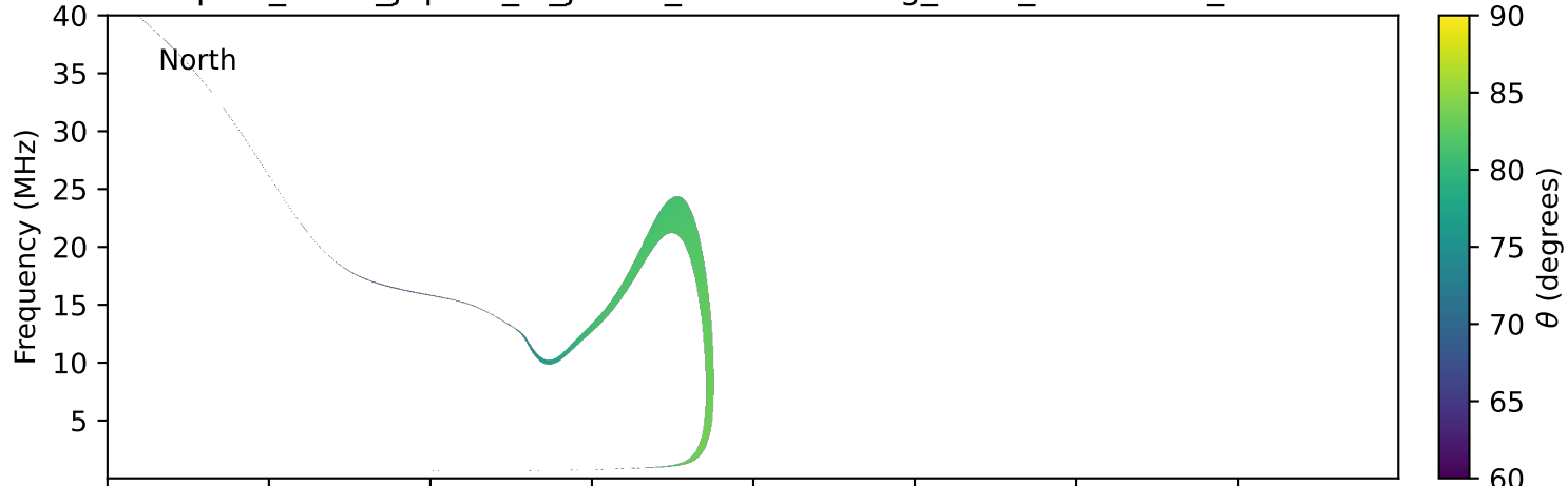
expres_earth_jupiter_io_jrm09_lossc-wid1deg_3kev_19770223_v11.cdf
