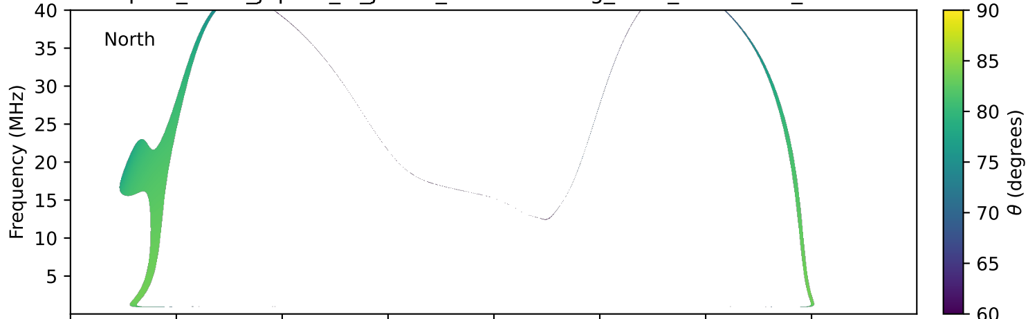
expres_earth_jupiter_io_jrm09_lossc-wid1deg_3kev_19770219_v11.cdf
