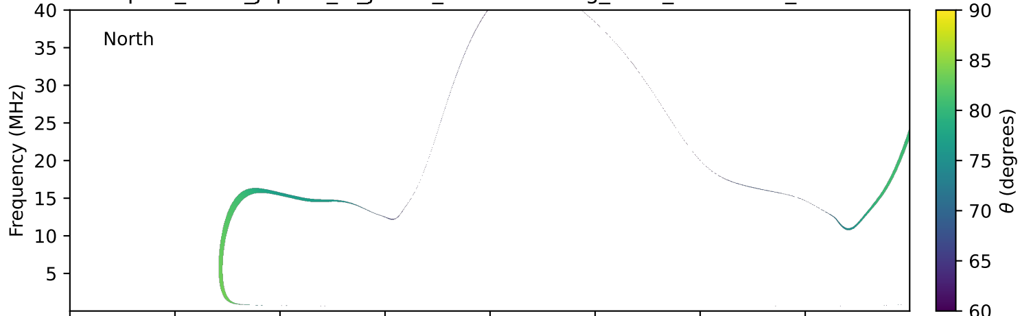
expres_earth_jupiter_io_jrm09_lossc-wid1deg_3kev_19770210_v11.cdf
