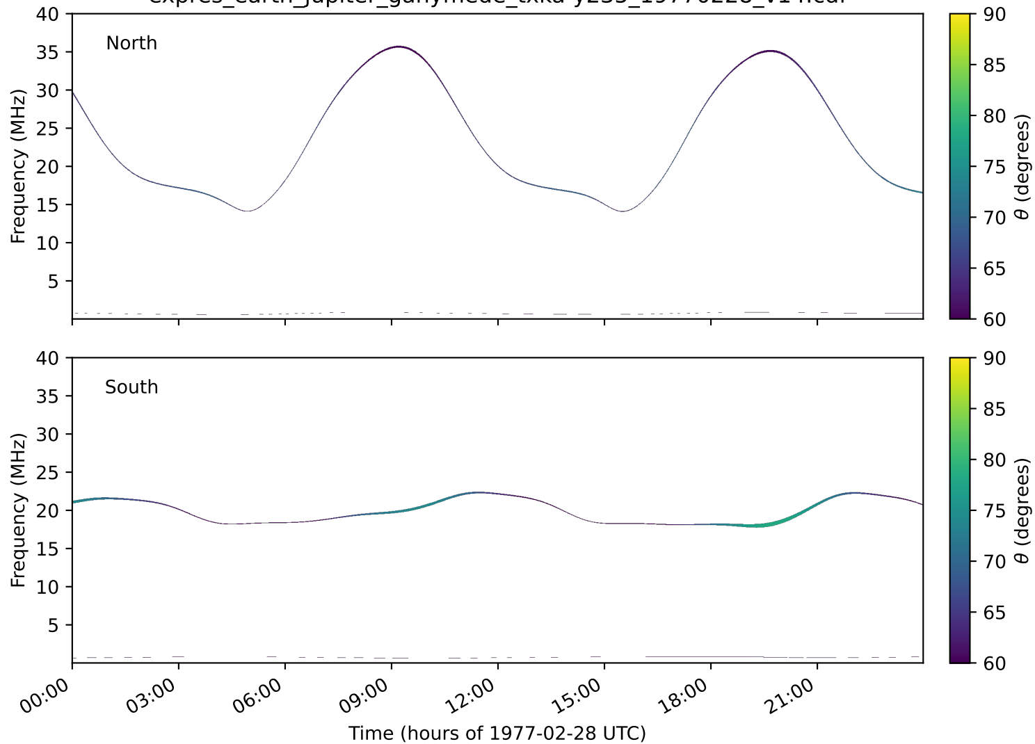
expres_earth_jupiter_ganymede_txka-y235_19770228_v14.cdf
