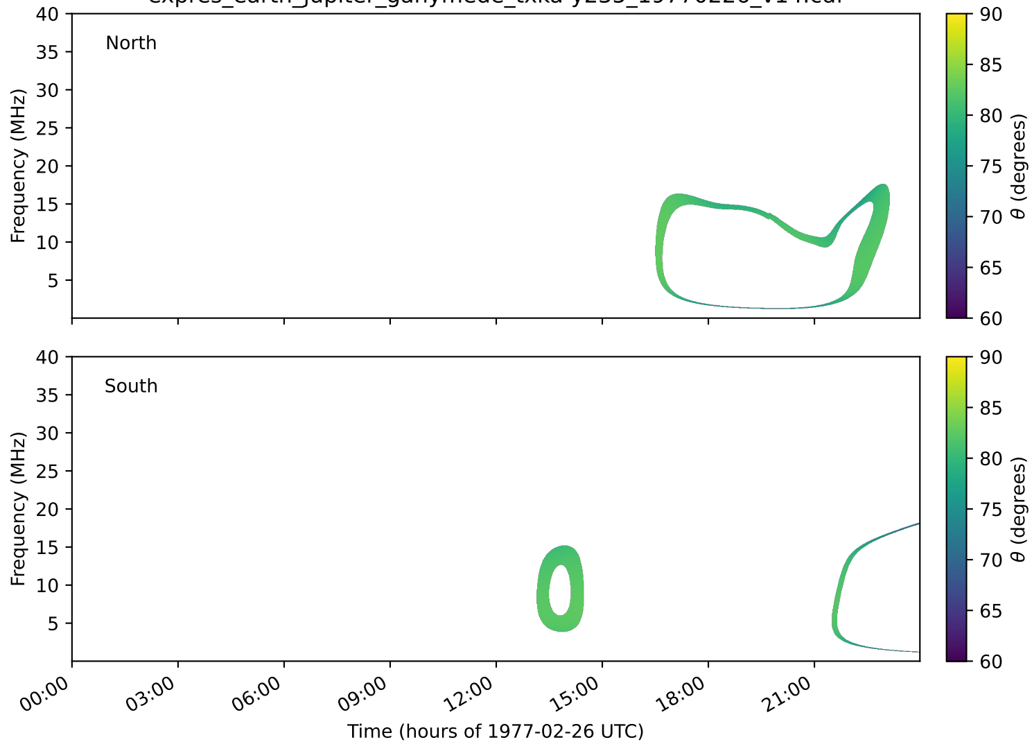
expres_earth_jupiter_ganymede_txka-y235_19770226_v14.cdf
