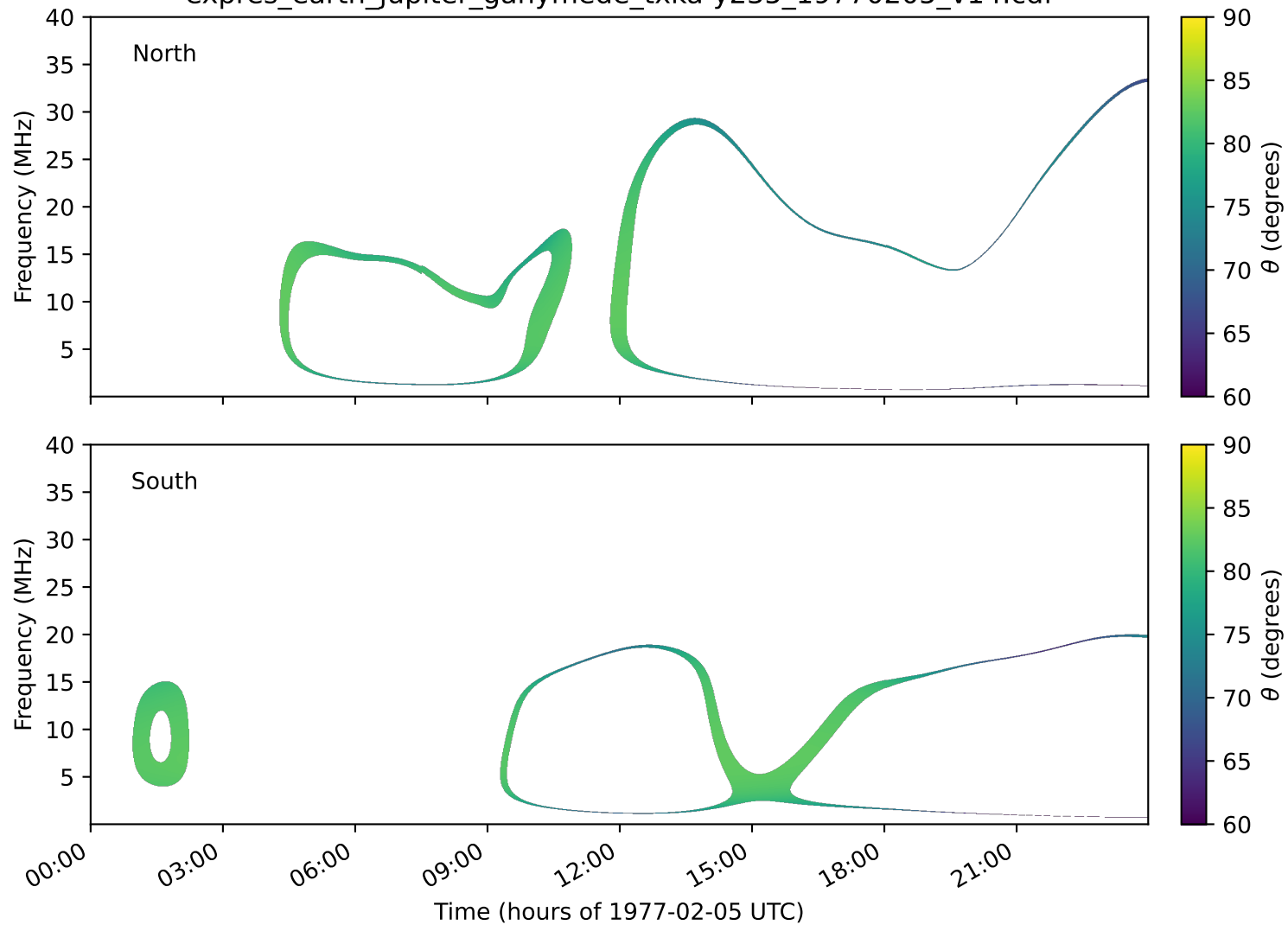
expres_earth_jupiter_ganymede_txka-y235_19770205_v14.cdf
