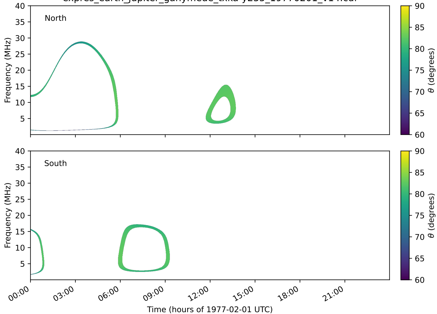
expres_earth_jupiter_ganymede_txka-y235_19770201_v14.cdf
