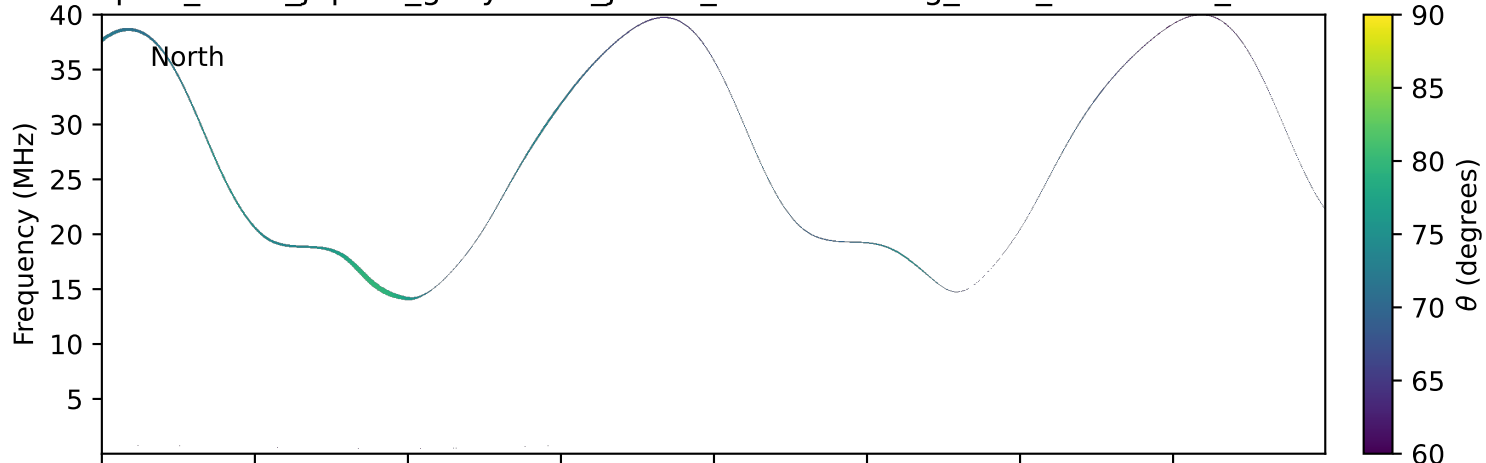
expres_earth_jupiter_ganymede_jrm33_lossc-wid1deg_3kev_19770213_v11.cdf
