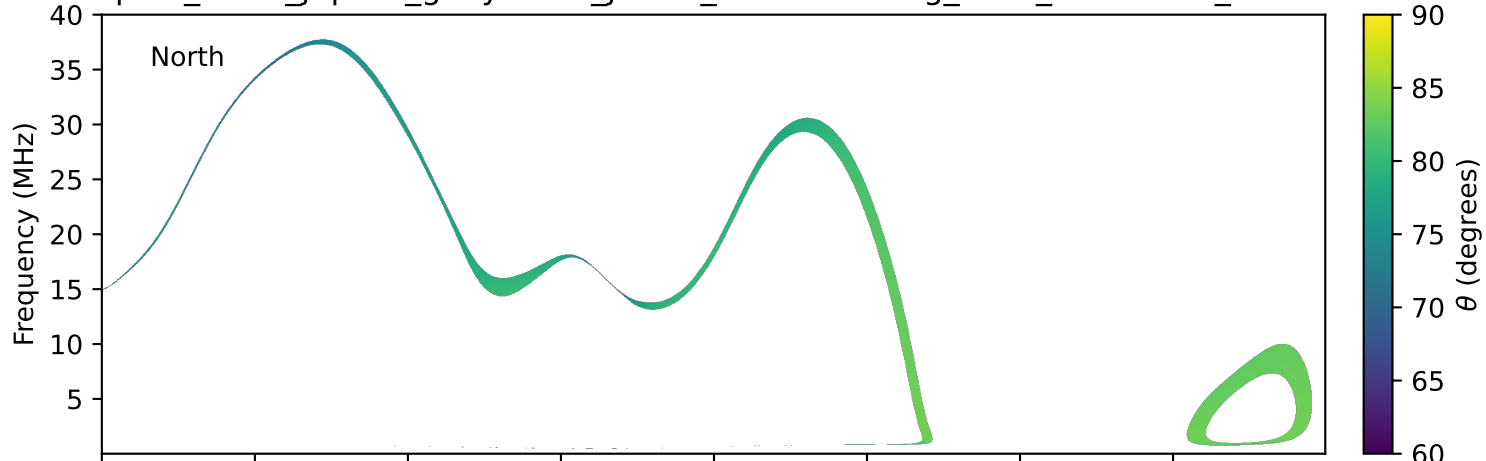
expres_earth_jupiter_ganymede_jrm33_lossc-wid1deg_3kev_19770208_v11.cdf
